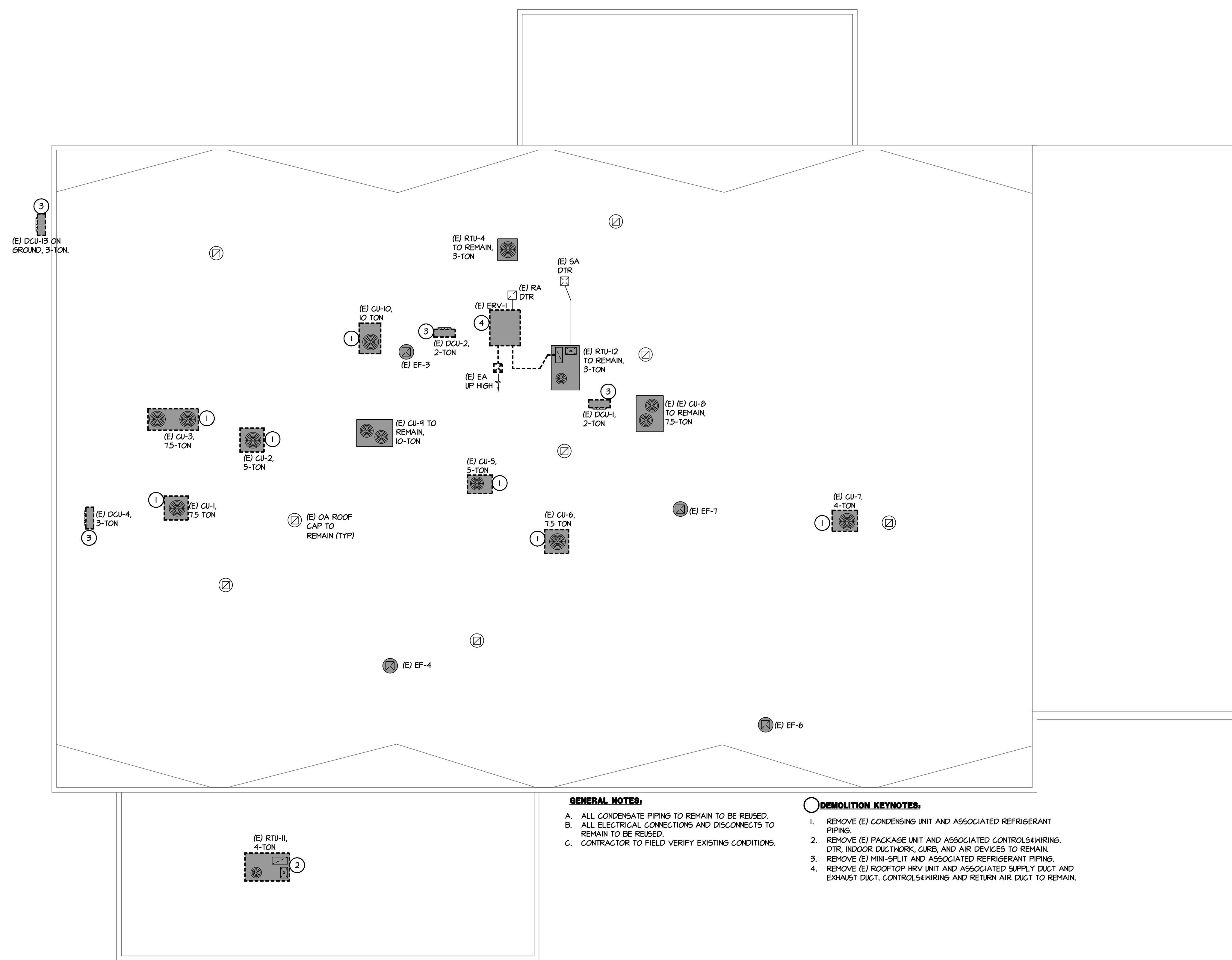
MECHANICAL DEMO ROOF PLAN SCALE: 1/8" = 1'-0"
