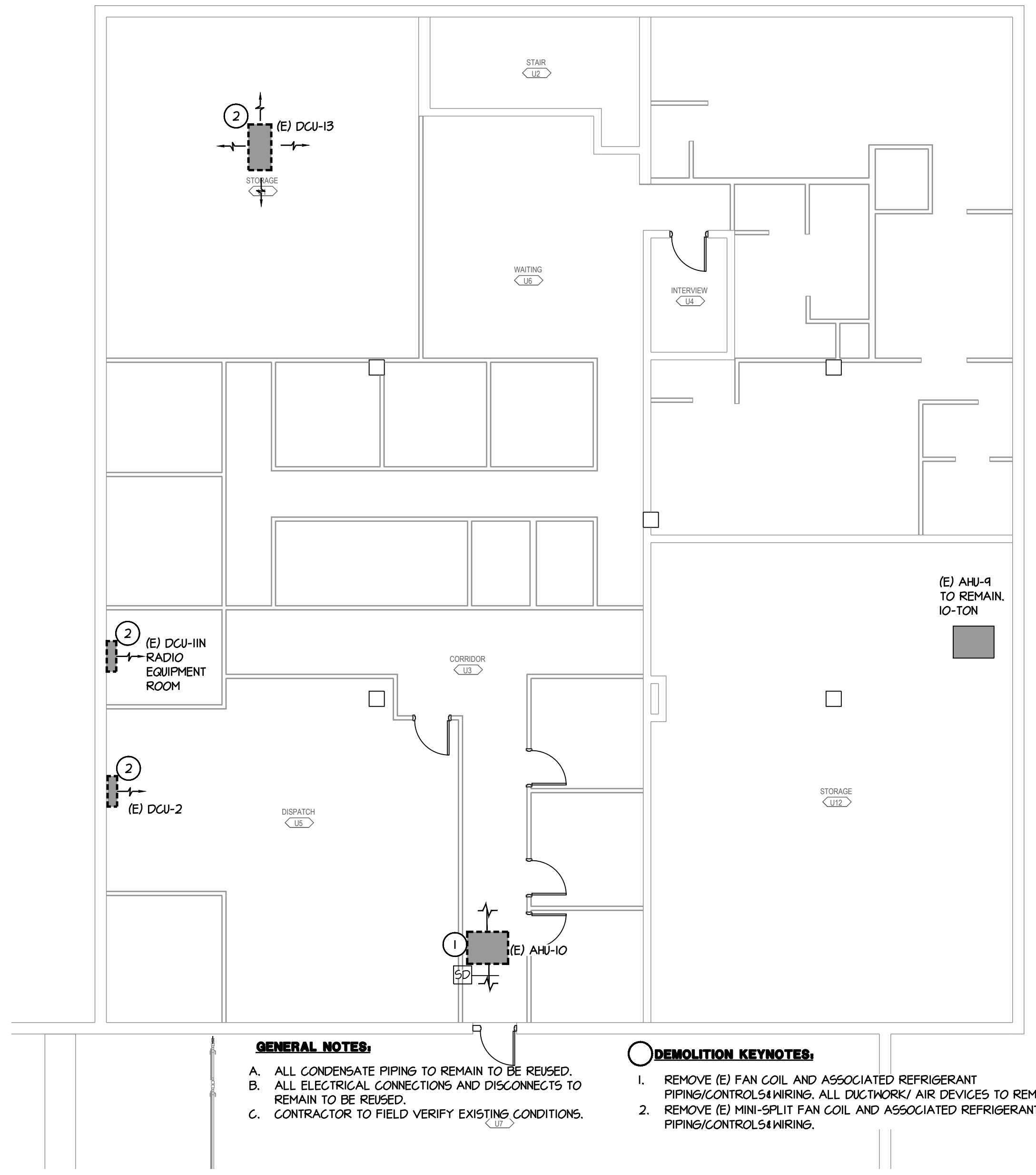
MECHANICAL DEMO BASEMENT PLAN SCALE: 1/8" = 1'-0" NORTH
